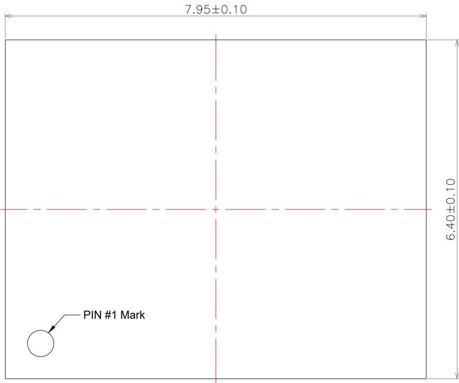
TOP VIEW
